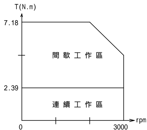
MA2-2200M
